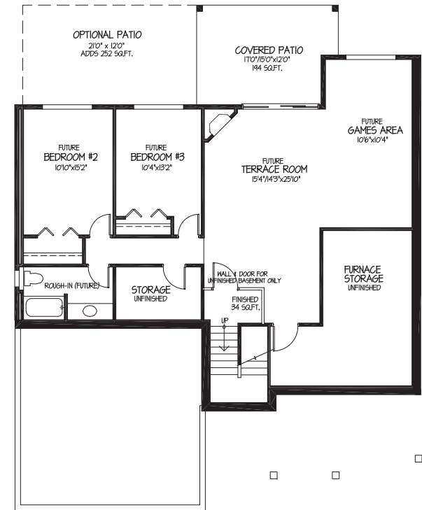
TERRACE LEVEL
